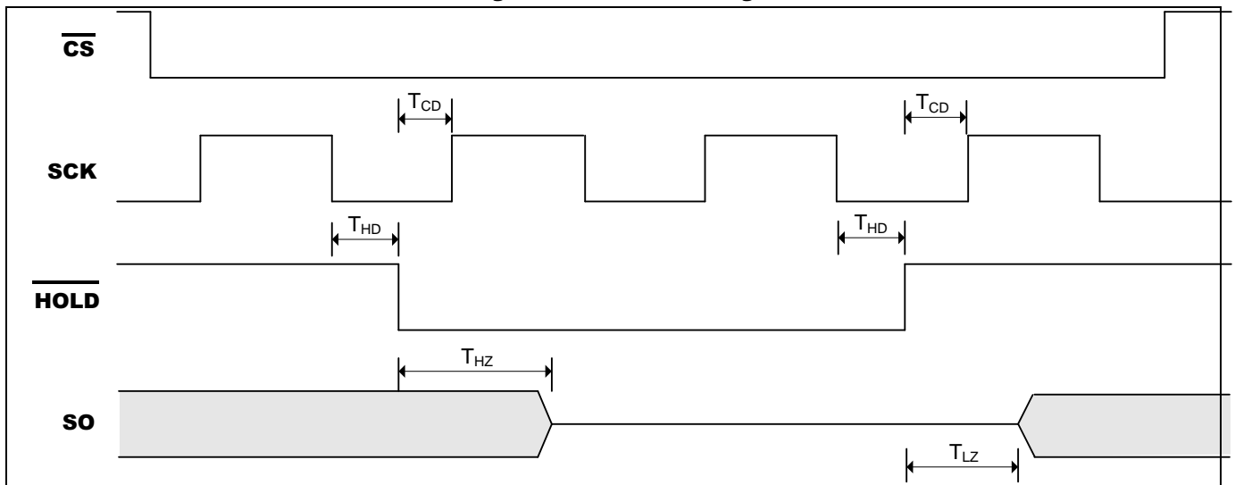
Figure 7-2. HOLD Timing
